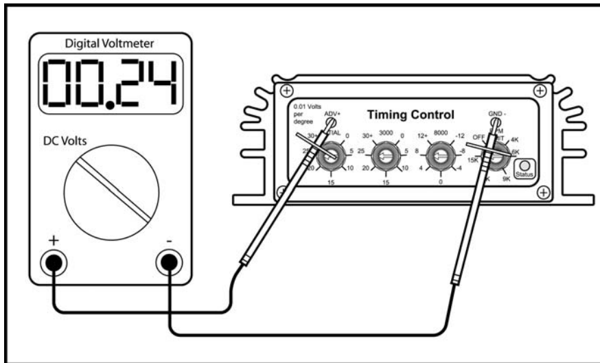
Figure 15 – Measuring timing with a digital voltmeter
