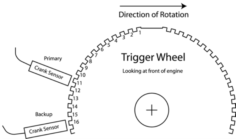
Figure 19 – Backup sensor location
